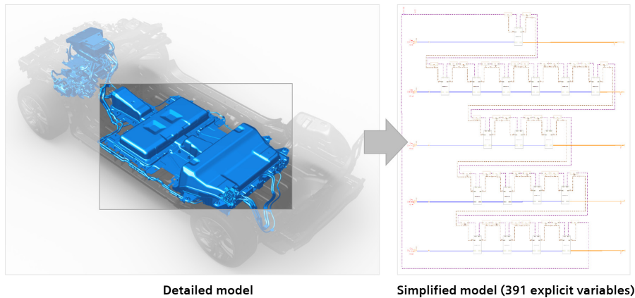
Figure 1. eCMP comparison between Simcenter Amesim and 3D model.
