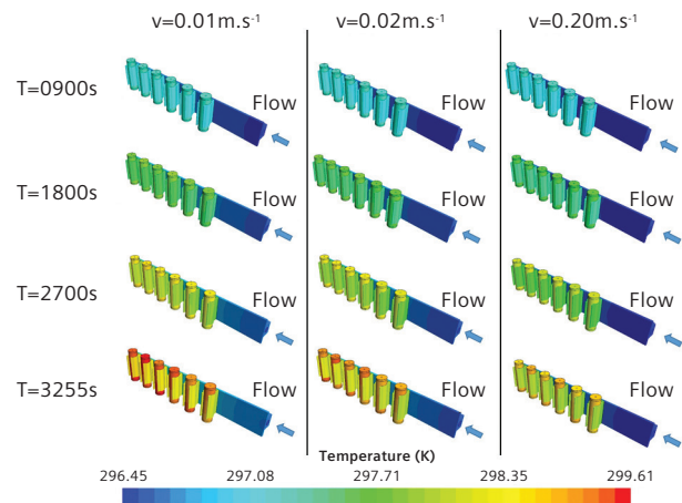
Figure 2: The temperature rise in the first set of series cells in the pack is a function of the .9 Celsius (°C) discharge rate and contact resistance of .0025 (m 2 .°K)/W.
