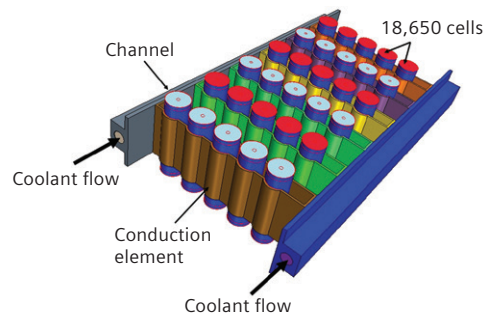
Figure 1: Geometry of the pack and the thermal management system.
